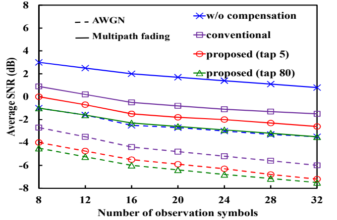
Fig 7. Average SNR vs number of observed symbols
