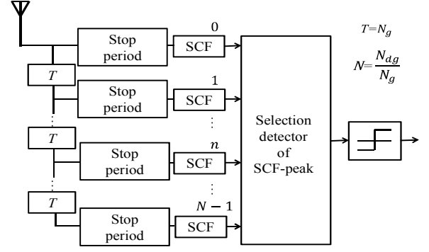
Fig 4. Proposed detector
