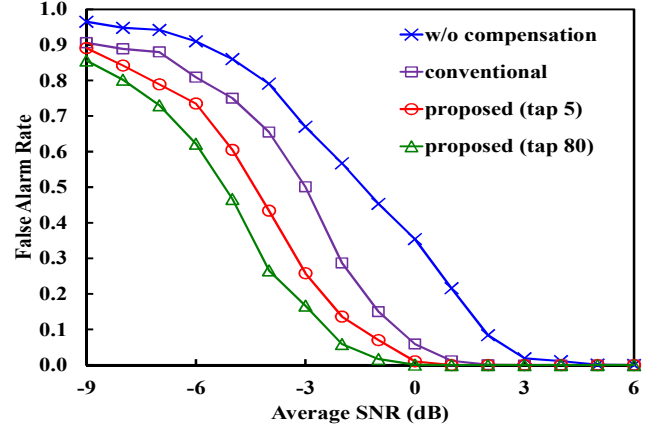
Fig 6. False alarm rate vs Average SNR under multipath fading channel
