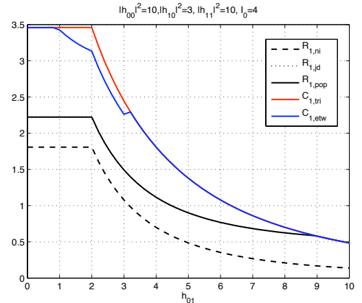
Fig. 4. Achievable rate and outer bounds vs the interference link gain of the primary user h_{01} .
