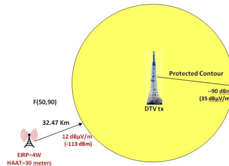
Fig. 9. Operation of fixed unlicensed devices in the framework of FCC regulations and ISDB-T standard.
