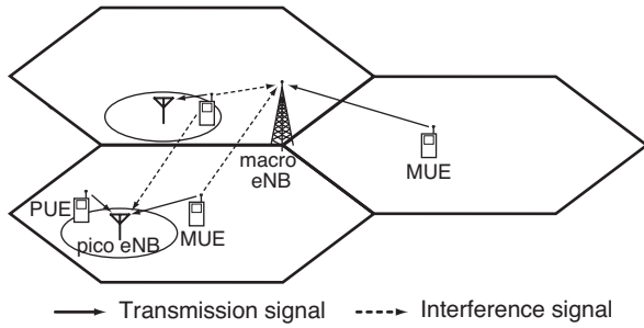
Fig. 1. System model of heterogeneous network in central macrocell site. In open access deployment, macro UEs are allowed make a handoff to the close-by pico eNB.
