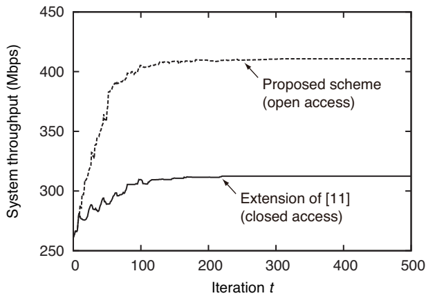
Fig. 3. Convergence of system throughput (4 pico eNBs/sector).
