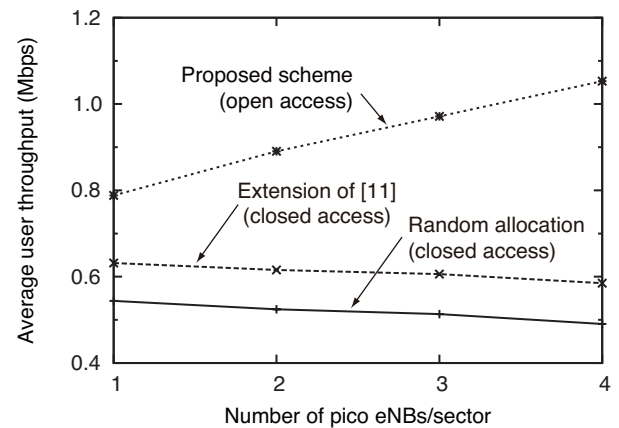
Fig. 5. Average macro UE throughput.
