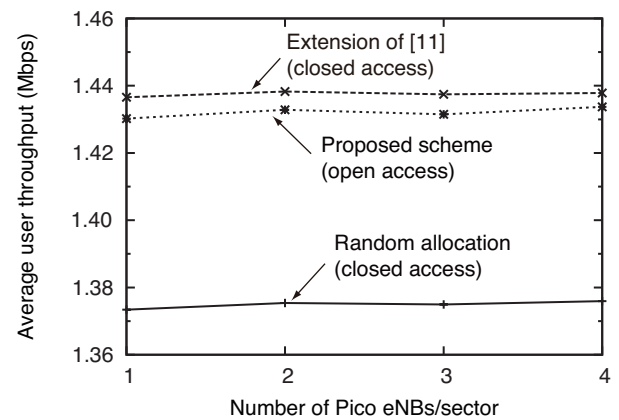
Fig. 6. Average pico UE throughput.
