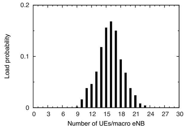
Fig. 4. Histogram of macro eNB load (4 pico eNBs/sector).
