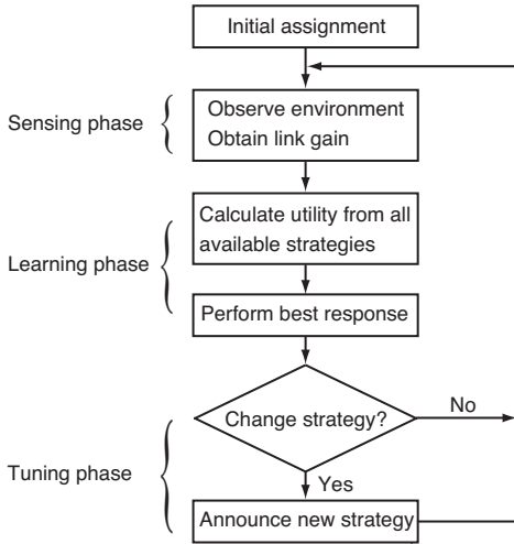
Fig. 2. Flowchart of the proposed self-organization scheme.
