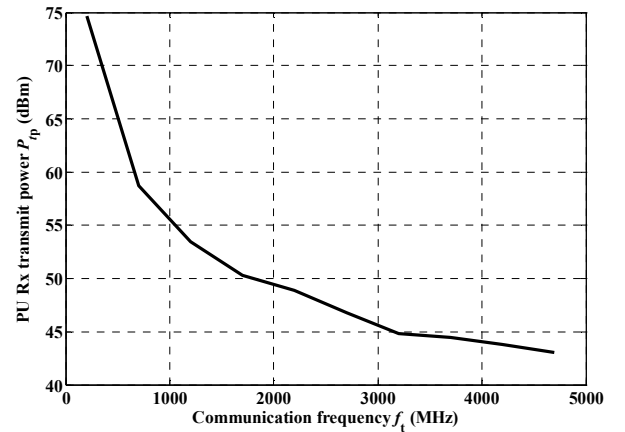
Figure 4. Impacts of path loss on required P_{\text{rp}} ( P = 95\% , R_2=8\text{km} ).
