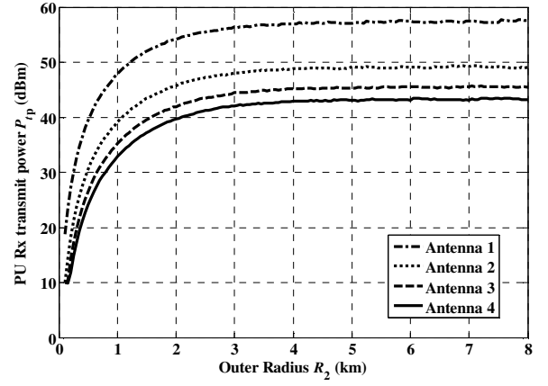
Figure 6. Diversity compensation for required P_p ( P = 95\% , f_c=1\text{GHz} ).
