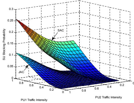
Fig. 8. SU blocking probability under SAC and JAC
