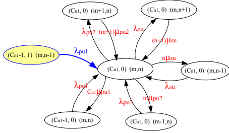
Fig. 4. Events analysis: PU1/SU arrival and departure
