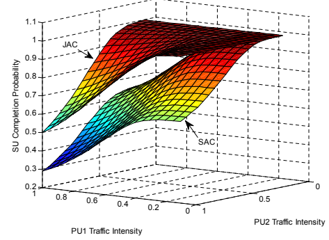
Fig. 10. SU completion probability under SAC and JAC
