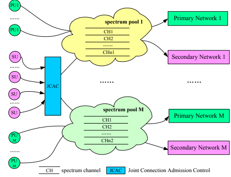
Fig. 2. Co-operative CRNs model with Joint Admission Control
