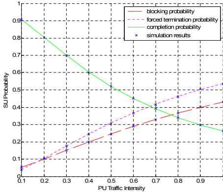
Fig. 1. Performance under Separate Admission Control
