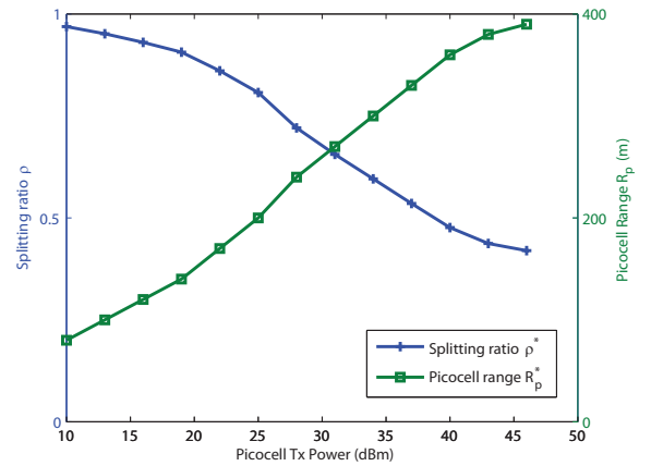
Figure 5. Optimal spectrum splitting ratio \rho^* and picocell range R_p^*
