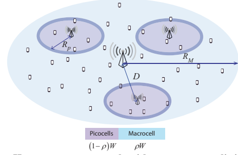
Figure 1. Heterogeneous network with a spectrum splitting model
