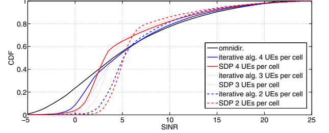
Fig. 5: Cumulative distribution function (CDF) of the SINR.
