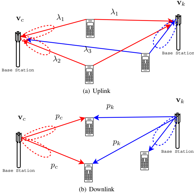
Fig. 1: UL-DL relation
