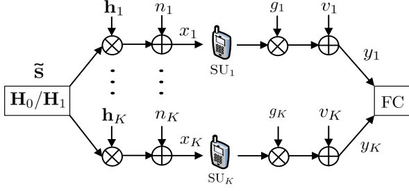
Fig. 1. Cooperative sensing in the secondary network with K SUs and FC at time instant m . antennas at the PU. Assuming each SU has a single receive antenna and denoting \mathbf{h}_k(m) \in \mathbb{C}^{1 \times N_t} as the stationary Rayleigh fading channel from the PU to the k th SU at the m th instant, we obtain the matrix \mathbf{H}(m) = [\mathbf{h}_1(m)^T, \dots, \mathbf{h}_K(m)^T]^T . The signal part received by the SUs at the m th instant is
