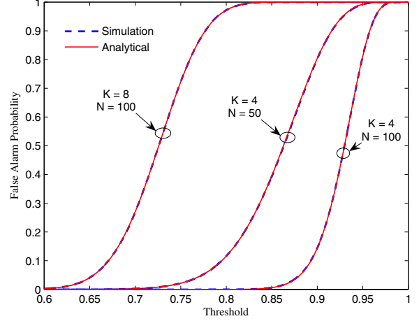
Fig. 1. False alarm probability: analytical versus simulation.
