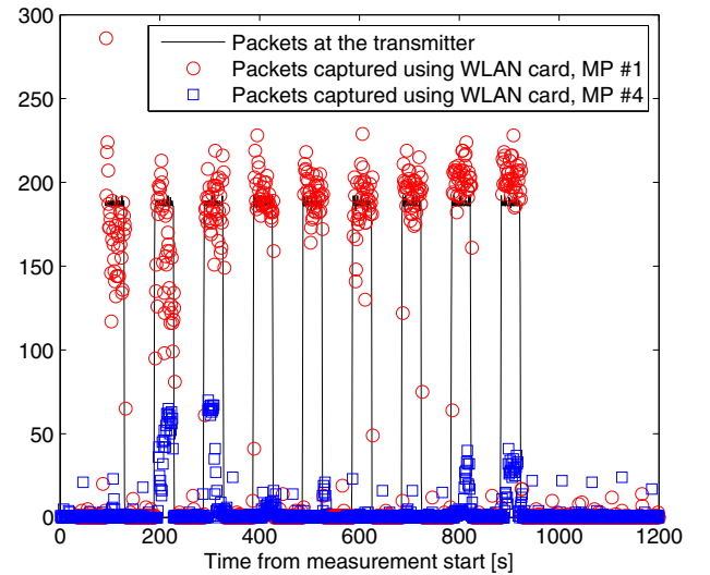
Fig. 4. Transmitter at MPs #1 and #4, Wireshark IO-results at the transmitter and the receiver (sensing laptop).
