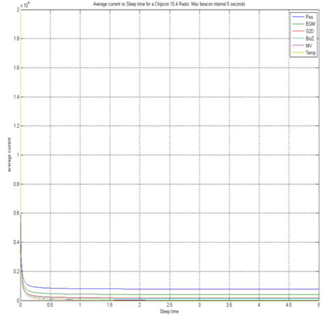
Figure 2 Decrease in average current as duty cycle increases for all sensors
