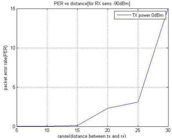
Figure 5 PER vs distance simulation
