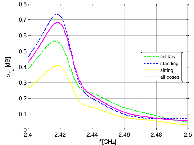
Figure 6. Input reflection coefficient (standard deviation).
