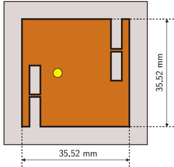
Figure 1. Patch antenna [10].
