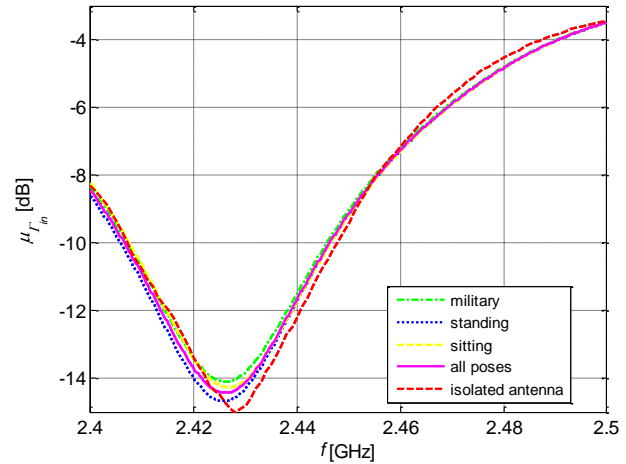
Figure 5. Input reflection coefficient (average).
