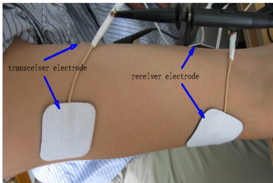
Figure 6. Measurement setup
