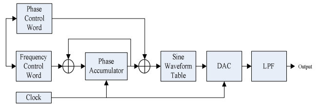
Figure 3. The function diagram of the AD9854
