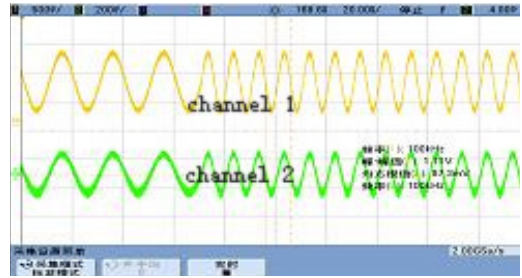
Figure 7. Output waveform of IBC transmitter
