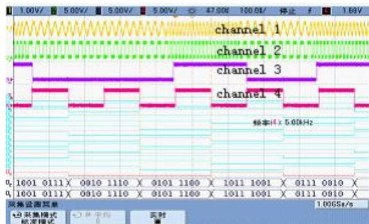
Figure 8. The waveform of IBC receiver
