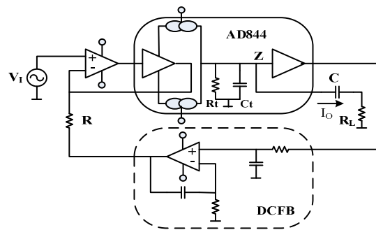
Figure 4. The circuit of the current source
