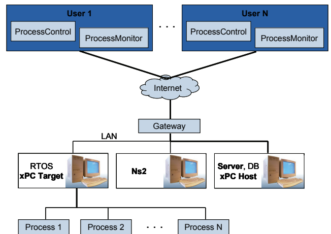
Figure 1. Architecture of the PiccSIM platform.
