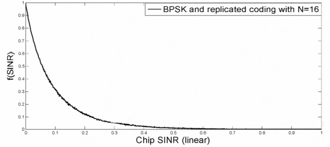
Fig. 1. f(\gamma) vs. chip level SINR
