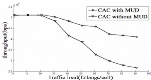
Fig. 6. Performance comparison of throughput with and without MUD
