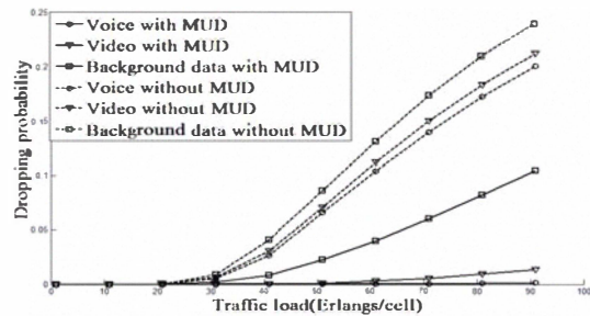
Fig. 8. Averaged dropping probability for different services in IDMA system with and without MUD
