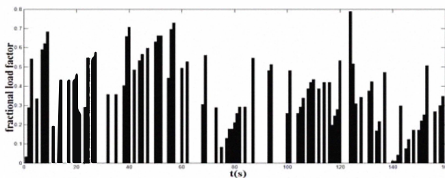
Fig. 5. The fractional load factor for one simulation
