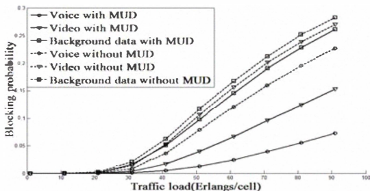
Fig. 7. Averaged blocking probability for different services in IDMA systems with and without MUD
