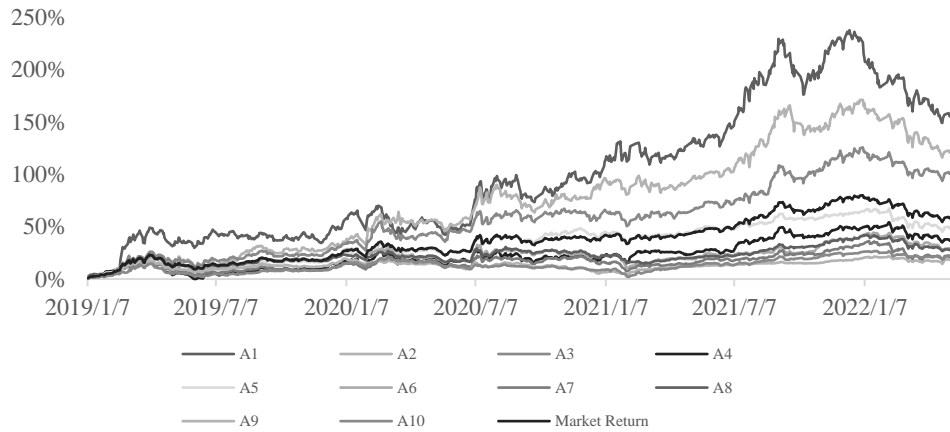
Figure 4 Weighted mean group back-test results
