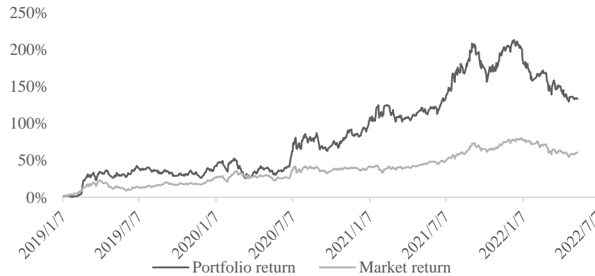
Figure 5 Long/short portfolio yield profile (bond balance weighted)
