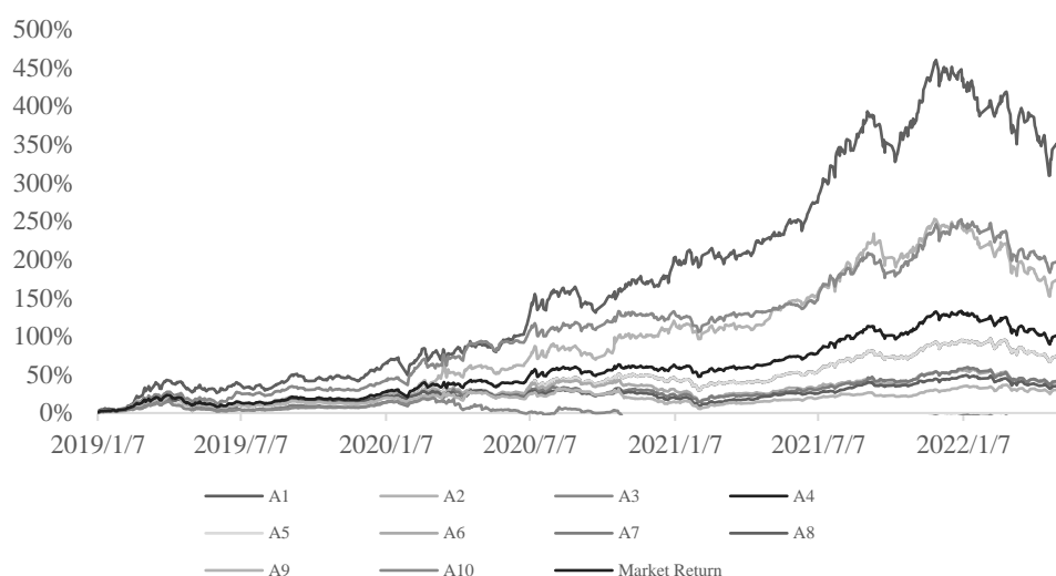
Figure 2 Arithmetic mean grouping back-test results
