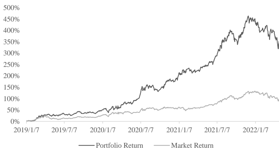
Figure 3 Arithmetic mean long-short portfolio return results
