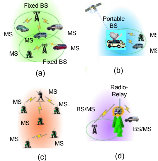
Fig. 2 Use cases of PBB system.
