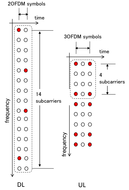
Fig. 5 Pilot symbol assignment for mode 1 (FFT size: 1024).
