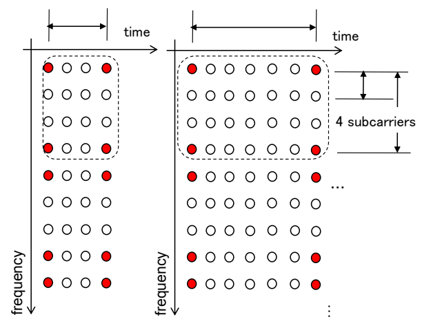
Fig. 6 Pilot symbol assignment for mode 2 (FFT size: 1024).
