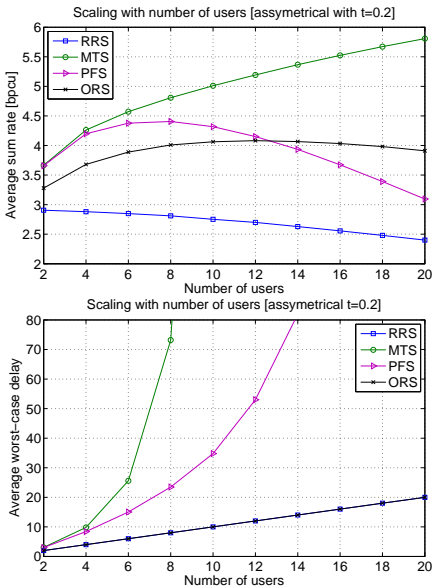
Fig. 3. Average sum rate and worst-case delay over number of users for asymmetrically distributed users.
