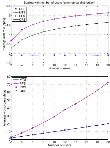
Fig. 2. Average sum rate and worst-case delay over number of users for symmetrically distributed users.
