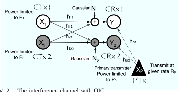
Fig. 2. The interference channel with OIC.
