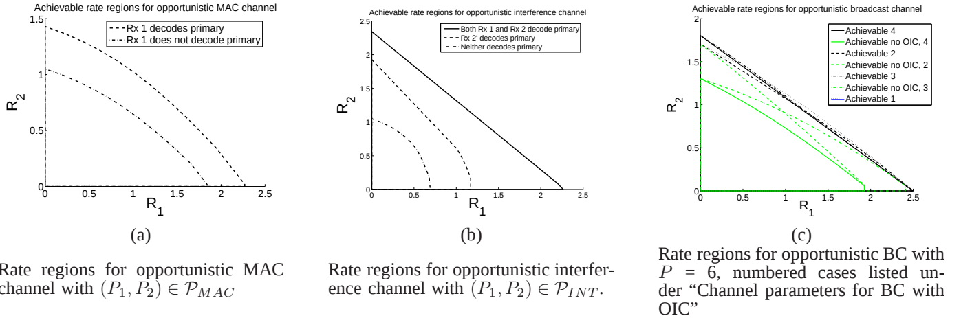
Fig. 4. Impact of opportunistic interference cancellation.
