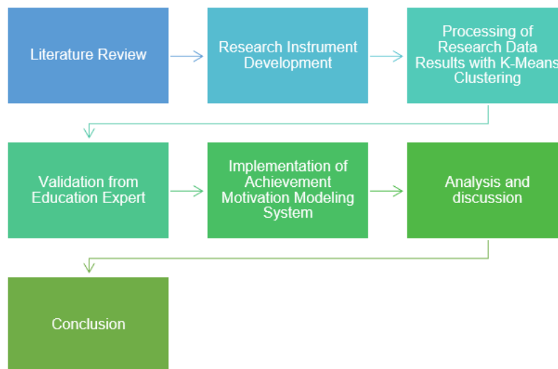
Fig. 1. Research Methodology
