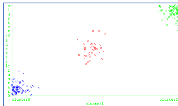
Fig. 3. Classification 10 fold
