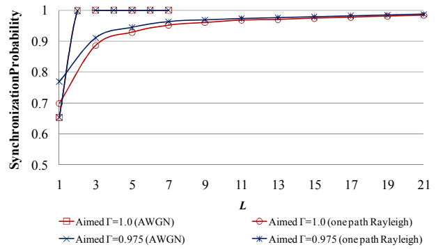
Fig.4 Synchronization probability vs. L of (7), \text{SNR}=-20\text{dB} .
