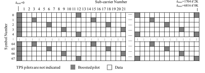
Fig.1 Locations of scattered boosted sub-carriers in DVB-T OFDM symbols ([10]). The horizontal axis represents the sub-carrier number (frequency) and the vertical axis represents the symbol number (time).
