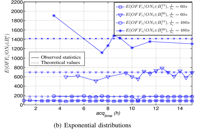
Fig. 3: Convergence of E(OFF_i/ON_i \in B_i^a) for some selected values of B_i^a
