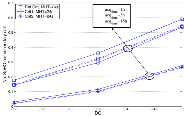
Fig. 5: Sensitivity to acq_{time} , dependent exponential data
