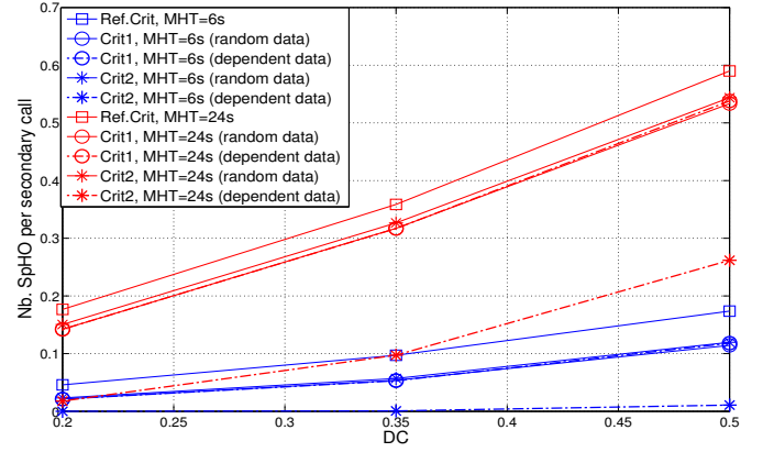
(b) Exponential Primary Activity Time Series
