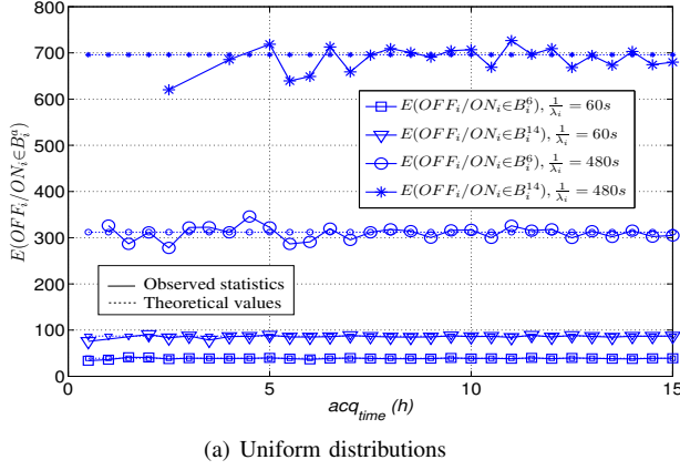
Fig. 3: Convergence of E(OFF_i/ON_i \in B_i^a) for some selected values of B_i^a
