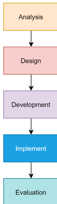
Fig. 1. ADDIE Framework
