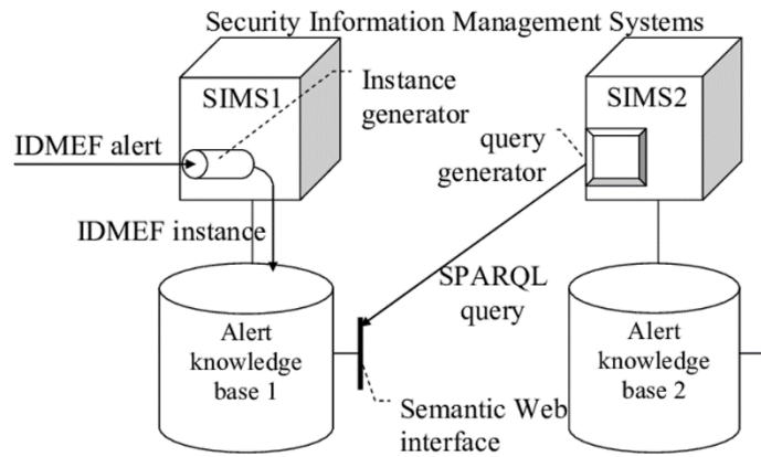
Fig 4. Semantic collaborative SIMS architecture
