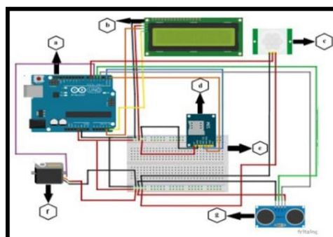
Fig 1. Block Diagram
