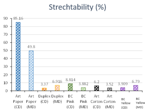
Fig. 7. The result test of stretchability.
