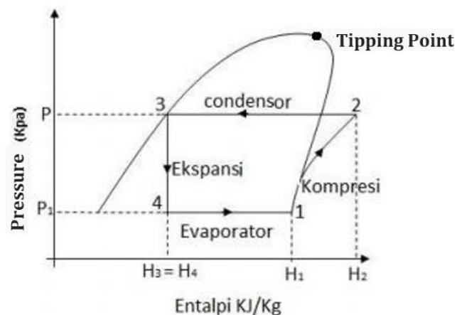
Fig 6. P-h Diagram
