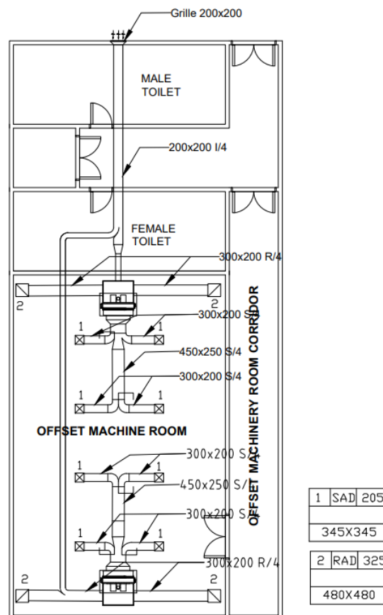
Fig. 9. Drawing of Cooling and Air Conditioning System Design in Engine Room
