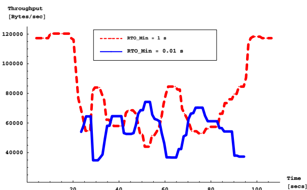
Figure 8: Throughput of two associations with different values for RTO-Min
