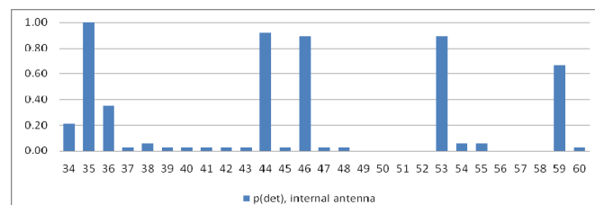
Fig. 10. Measured probability of DVB-T detection, n = 37 per channel, average distance to Espoo transmitter 15 km and 78 km to Tallinn transmitter.
