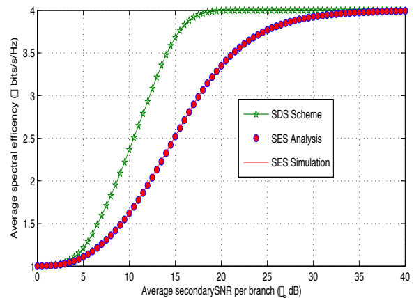
Fig. 5. Average spectral efficiency versus \overline{\gamma_s} (in dB).
