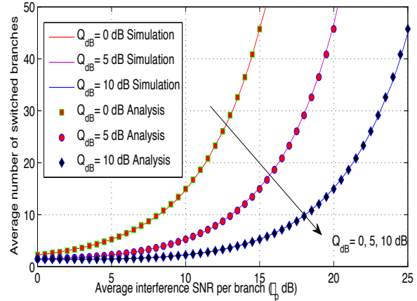
Fig. 4. Average number of switched branches versus \overline{\gamma_p} (in dB) for different levels of Q .
