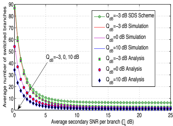
Fig. 3. Average number of switched branches versus \overline{\gamma_s} (in dB) for different levels of Q .
