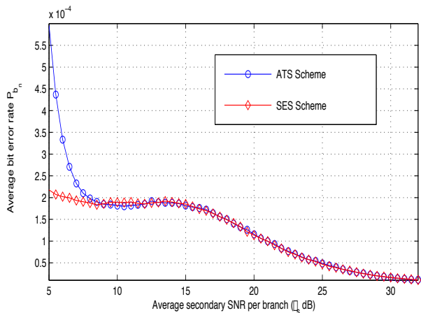
Fig. 6. Average BER versus \overline{\gamma}_s (in dB).
