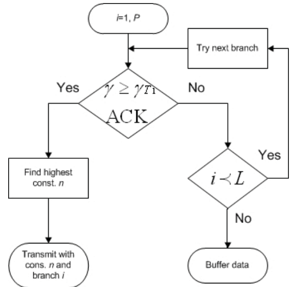
Fig. 2. Switching efficient scheme.
