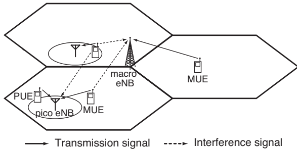
Fig. 1. System model of heterogeneous network in central macrocell site. In open access deployment, macro UEs are allowed make a handoff to the close-by pico eNB.
