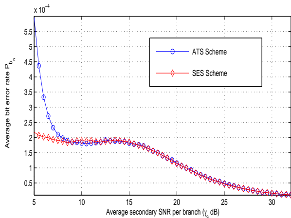
Fig. 6. Average BER versus \bar{\gamma}_s (in dB).
