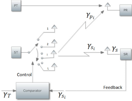
Fig. 1. System model.
