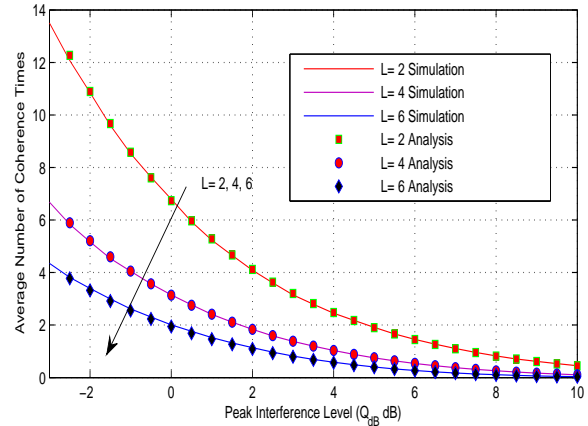
Fig. 7. Average number of slot times required before finding an acceptable branch versus the peak interference level Q_{dB} for \bar{\gamma}_{s,dB} = \bar{\gamma}_{p,dB} = 10 dB and for different values of L .
