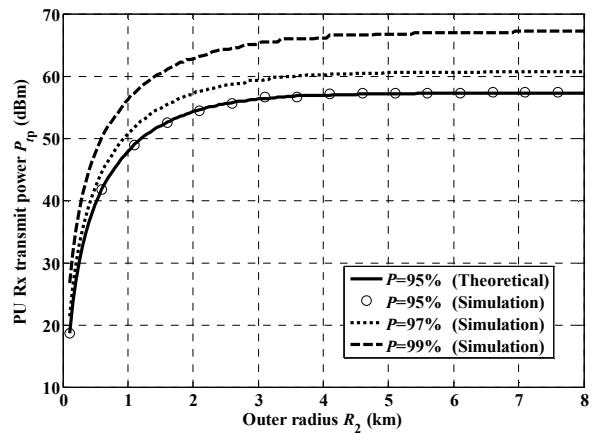
Figure 3. Theoretical and simulation results for interference avoidance ( for P from 95% to 99%, f_i=1\text{GHz} ).
