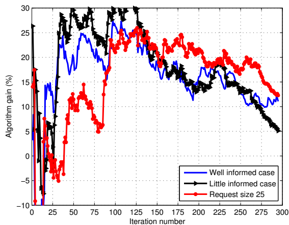
Fig. 3. Algorithm gain compared to the random choice of measurements
