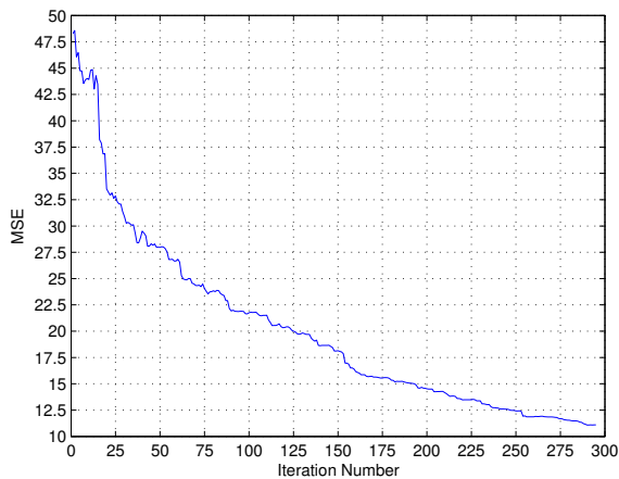
Fig. 2. Mean Square Error as measurements are added
