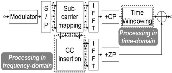
Figure 4. IA-PFT transmitter structure.
