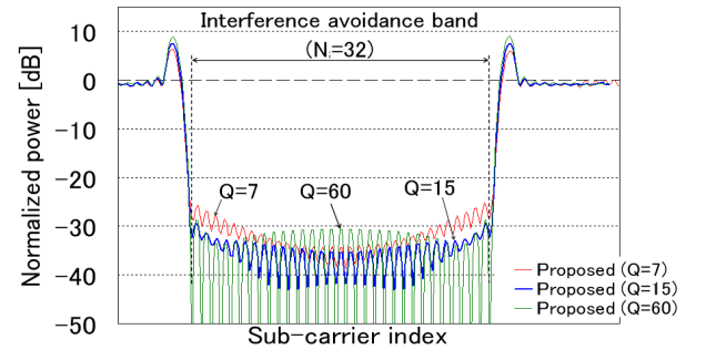
Figure 6. Power spectrum density of IA-PFT with variable Q .
