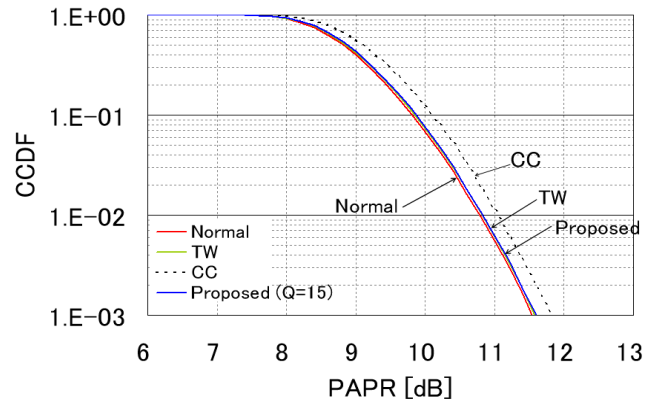
Figure 7. PAPR performance of IA-PFT.
