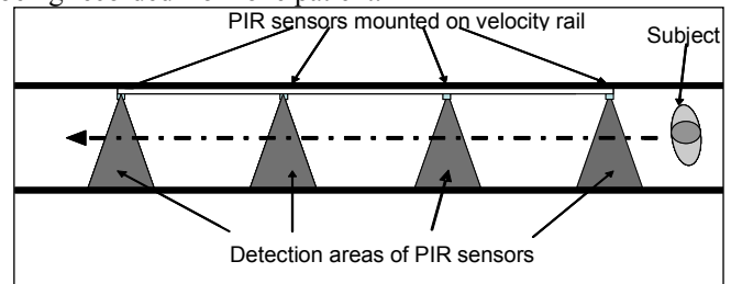
Fig. 1. Velocity Rail Schematic.
