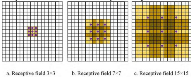
Figure 1. Expansion of receptive field due to dilated convolution
