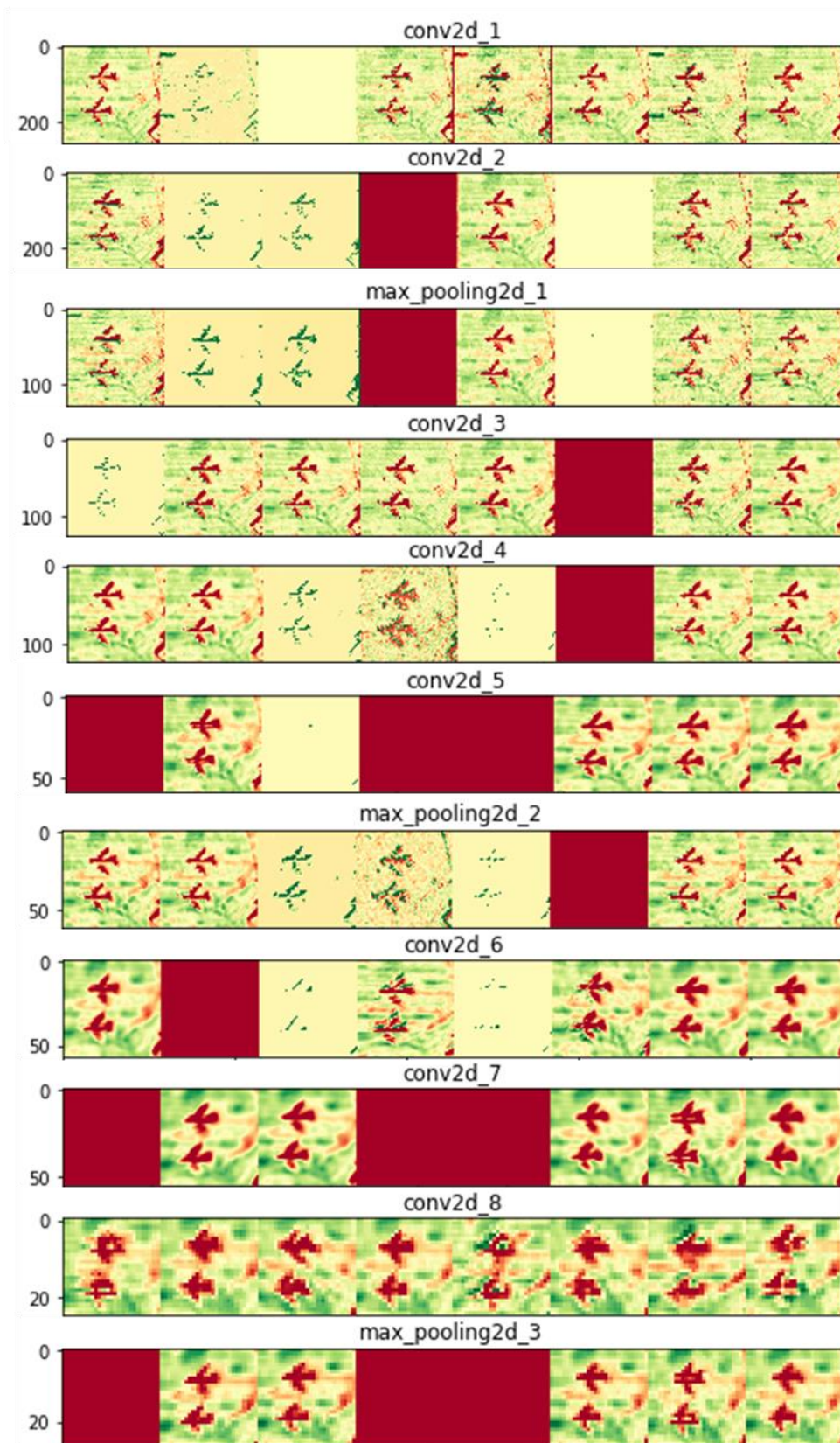
Figure 4. Feature visualization of optimized RSISC-16 Net Model
