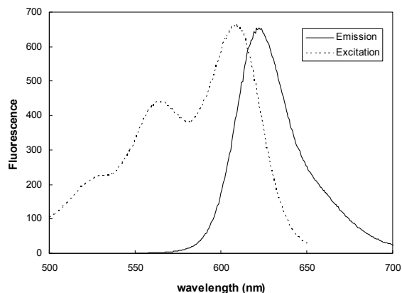
Figure 2. The excitation scan and emission scan of 15 \mu M quinizarin in the presence of 25 \mu M lithium.
