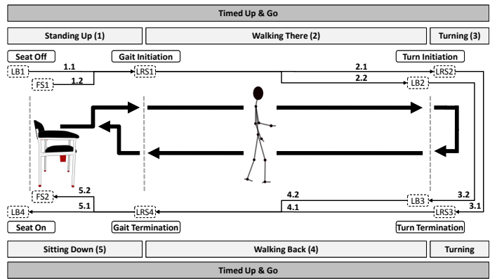
Fig. 1. aTUG Concept and Expansion Stages
