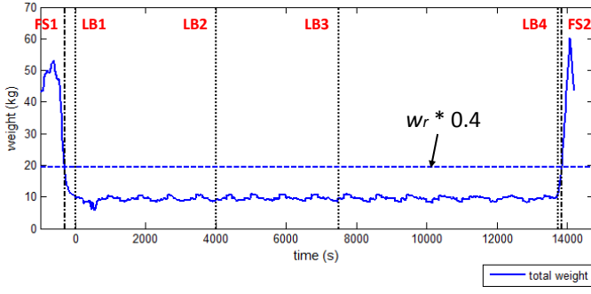
(a) Component Detection Using Force Sensors
