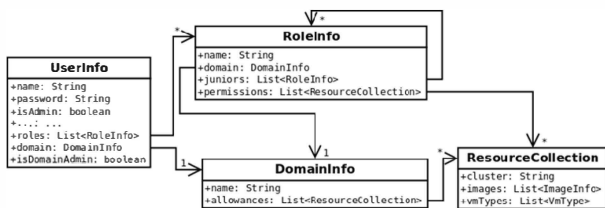
Fig. 3. RBAC Object Design
