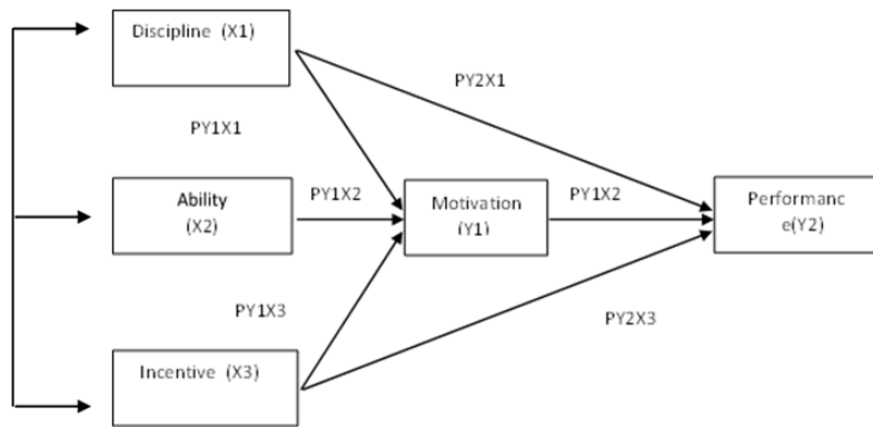
Fig. 1. Conceptual Framework
