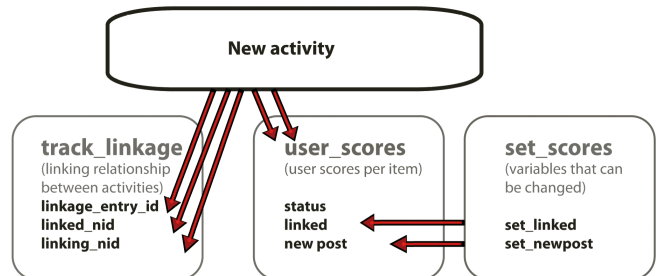
Figure 5. The scoring system in Drupal when creating an activity.
