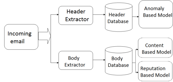
Figure 1. Block Diagram of Hybrid SPAM filter.
