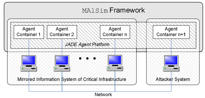
Figure 2: MAISim deployment.
