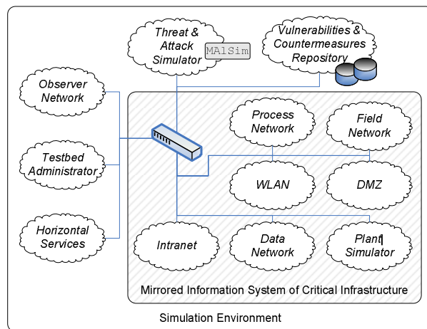
Figure 1: Simulation environment.
