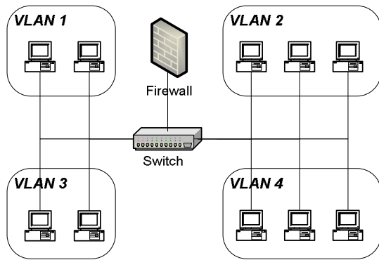
Figure 4: An exemplary setting of Threat and Attack Simulator network.
