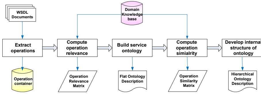
Fig. 1. The Ontology Construction Framework
