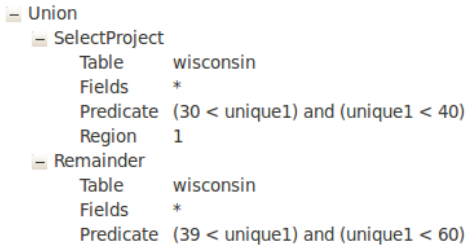
Fig. 5. Local Query Plan Tree
