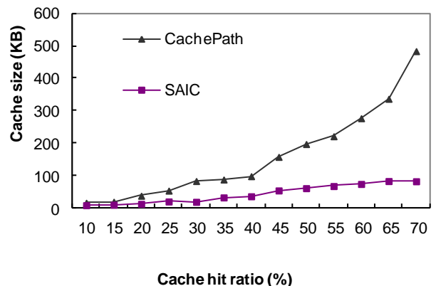
Figure 5. Comparison of cache space requirement.
