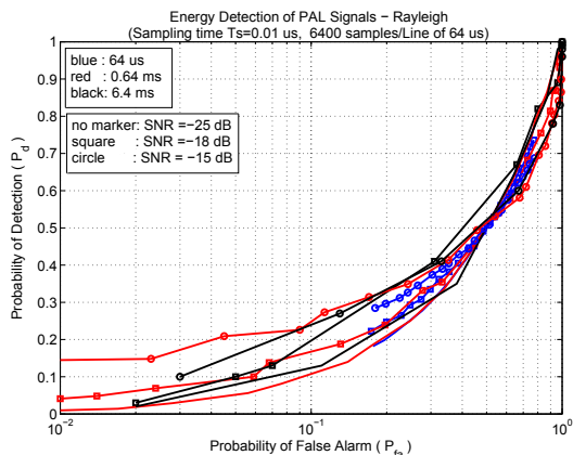
Fig. 10. Simulations: Probability of detection vs. probability of false alarm of PAL Sensing in Rayleigh fading channel based on EDM.
